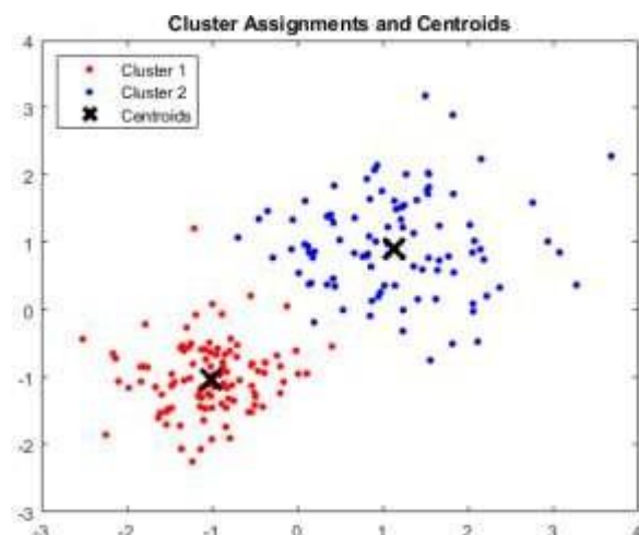
Figure 7: K-mean clustering
