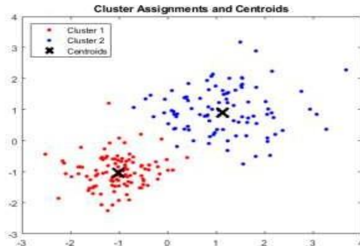
Figure 7: K-mean clustering
