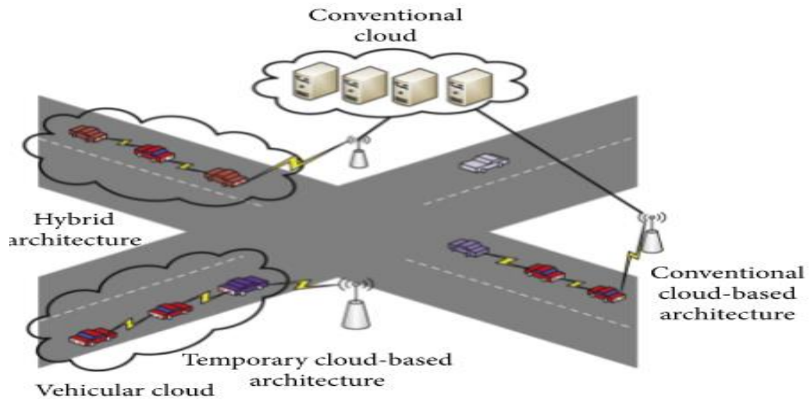
Figure 1.2 System Architecture
