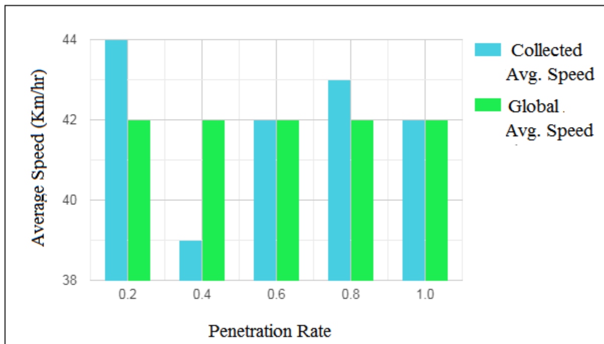
Figure 1.5 Medium Traffic Demand (Density = 50 Vehicle/Km)
