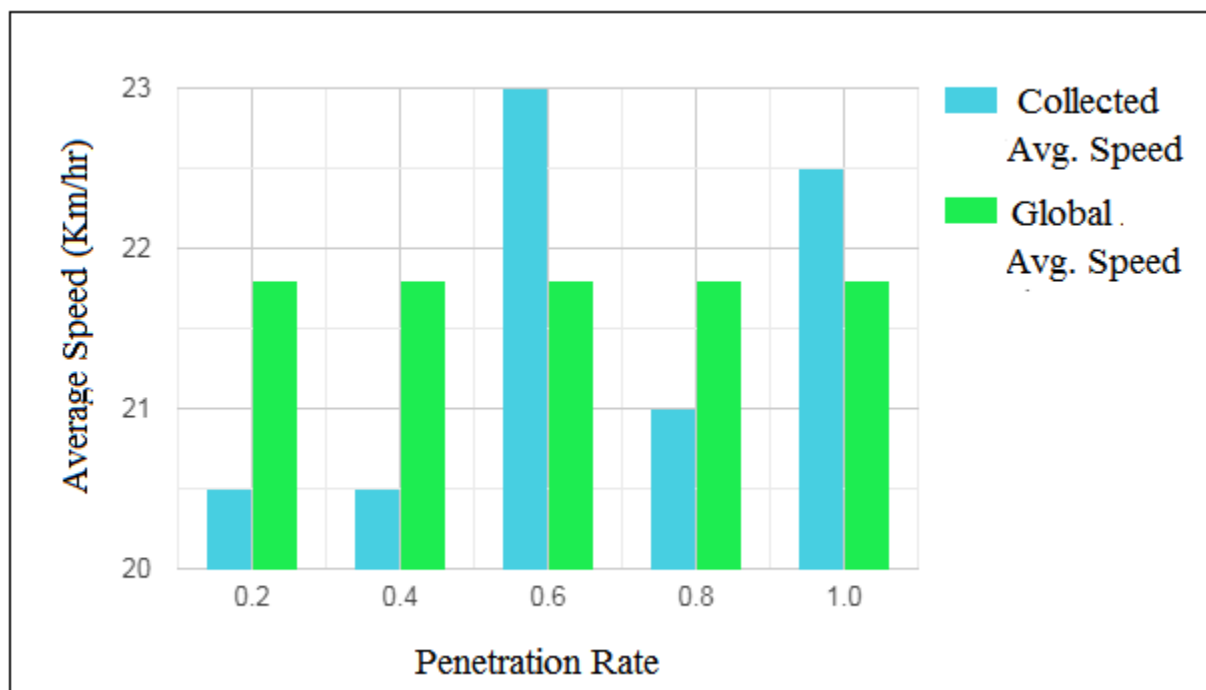
Figure 1.4 High Traffic Demand (Density = 70 Vehicle/Km)
